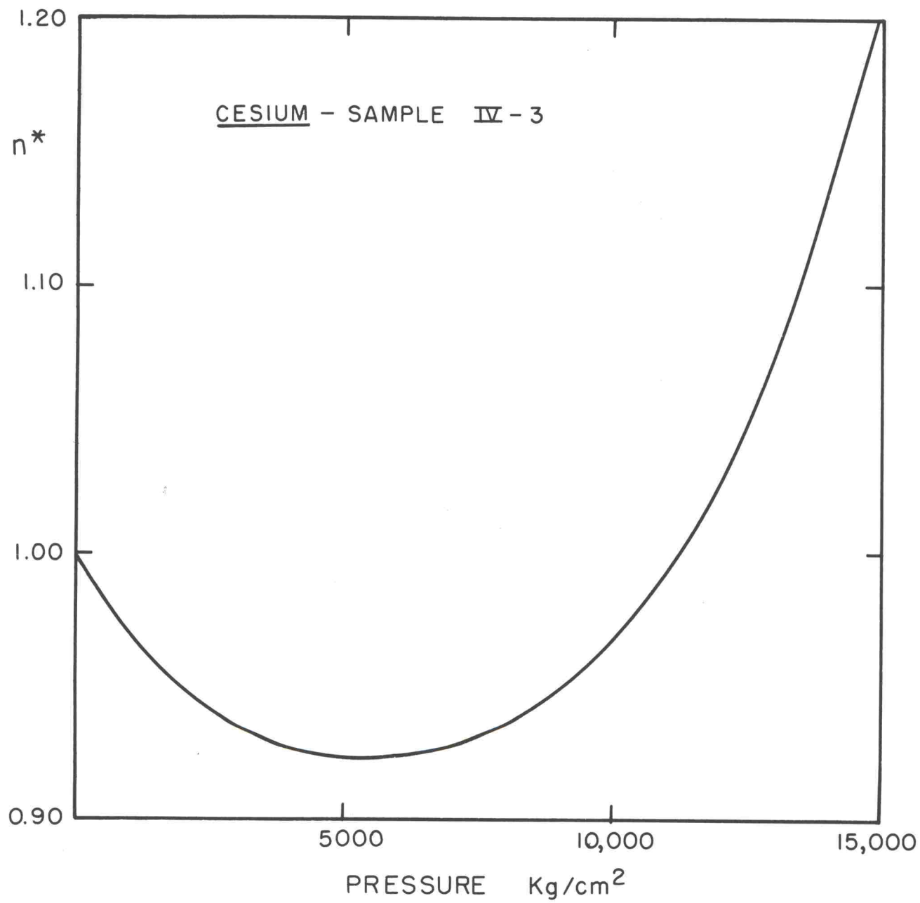
FIG. 3-14 n^* , NORMALIZED ELECTRONS/ATOM VS. PRESSURE
